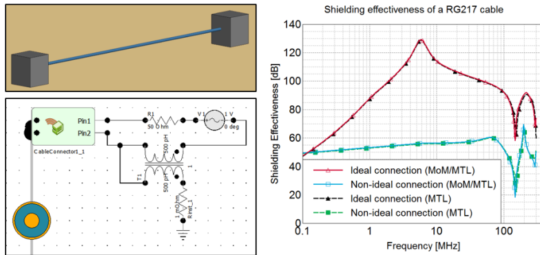
Figure 68: A non-ideal cable termination modelled using the new transformer component.
