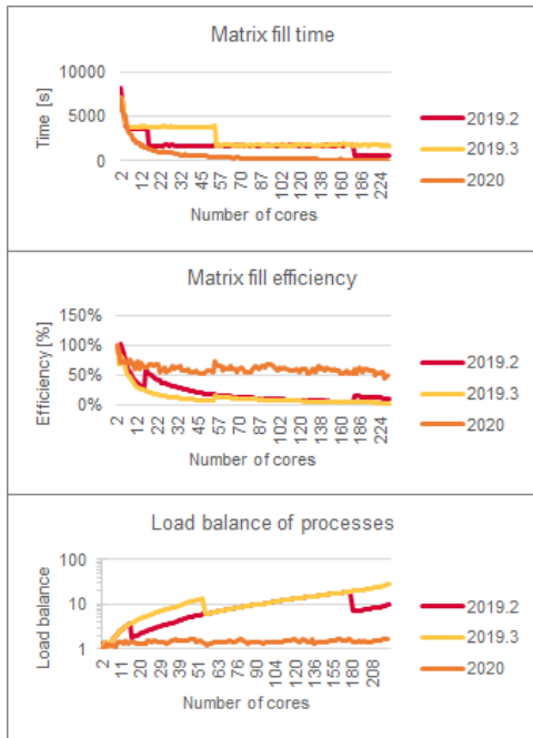
Figure 60: A comparison of the parallel scaling performance of the MLFMM between versions 2019.2, 2019.3 and 2020.
