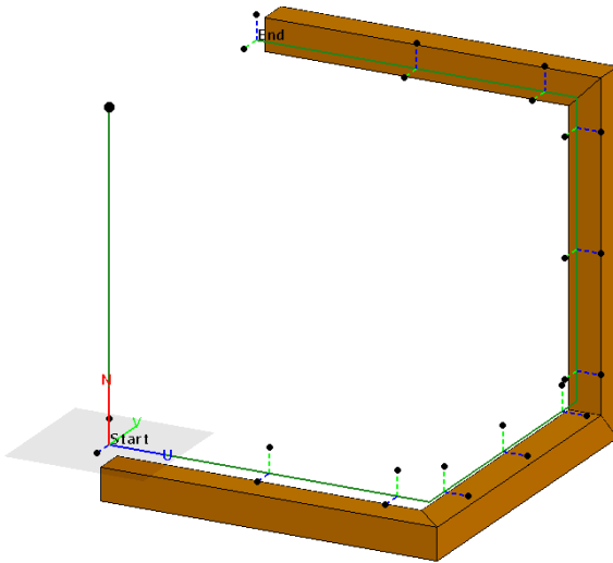
Figure 85: A reference direction can be defined to specify the orientation of a cable.
