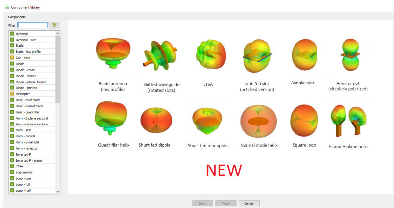
Figure 54: A selection of new antennas in the CADFEKO component library.
