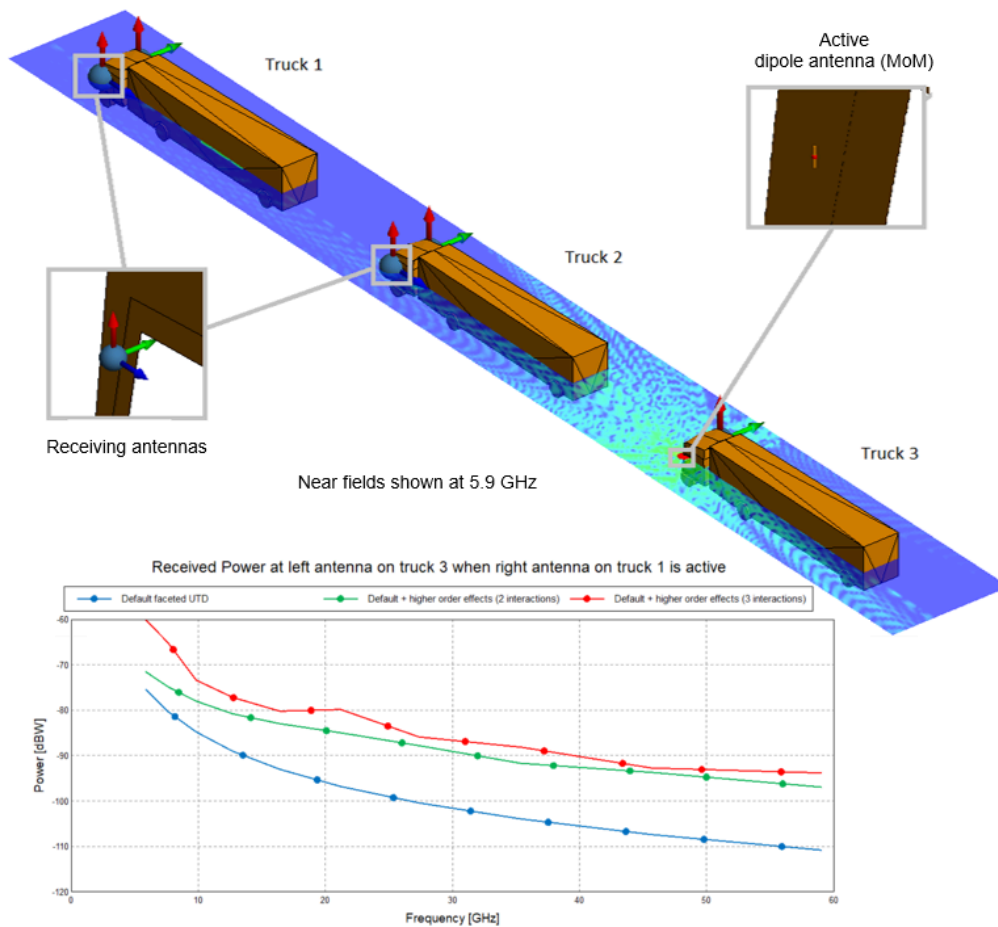
Figure 36: Faceted UTD coupled with MoM used to analyse the field distributions and antenna coupling for rear-view mirror mounted communication antennas in a set of platooning trucks at different frequencies. Multiple interactions and the inclusion of higher-order effects result in more accurate calculation of coupling between certain combinations of antennas.
