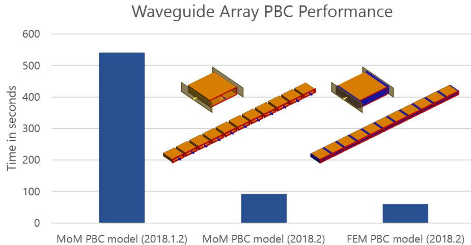
Figure 74: An 11x11 waveguide array solved at 1.645 GHz. The image shows the performance of the MoM PBC array solved with Altair Feko 2018.1.2 compared to the MoM PBC array solved with Altair Feko 2018.2 and the FEM PBC array solved with Altair Feko 2018.2. The PBC unit cells for the MoM and FEM models are shown as inserts with the 3D views of the models. The simulations were completed on a standard desktop computer (Intel® Core™ i5-4690 CPU @ 3.50GHz).
