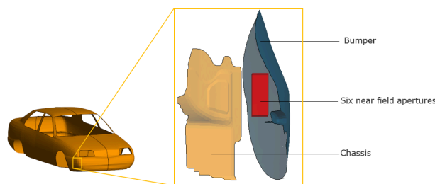
Figure 71: Side view of a radar antenna placement using 6 near field apertures, located in between the bumper and chassis.
