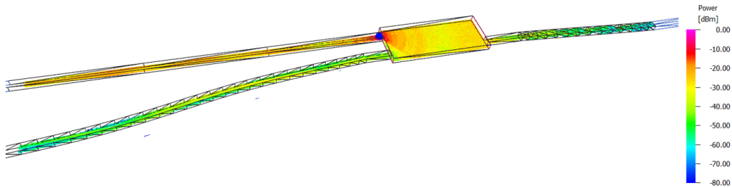
Figure 43: An example of multiple tunnels and a station.
