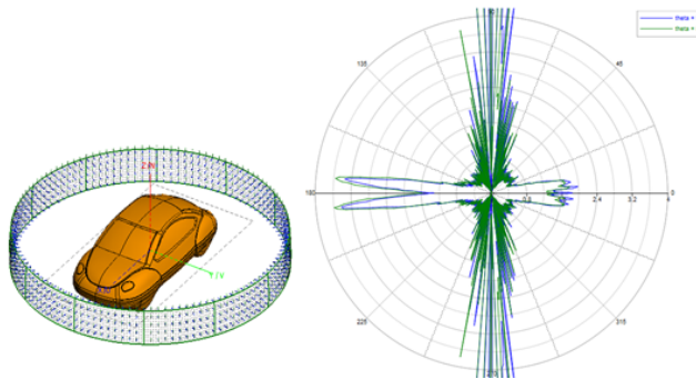
Figure 73: Feko-calculated RCS information can be included in a WinProp simulation through .ffe file import.
