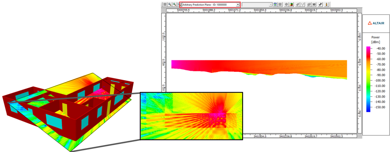
Figure 11: Examples of arbitrary prediction planes that are now available in the prediction plane drop-down list. Left: Arbitrary plane in an indoor scenario in the 3D view and new 2D view; Right: A vertical prediction plane used in the PE model.
