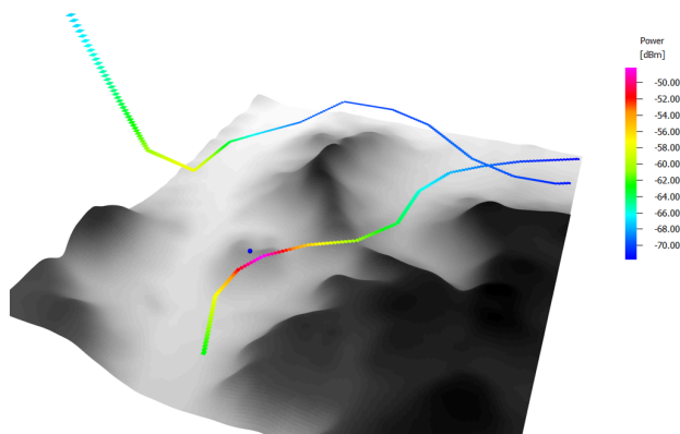
Figure 69: Trajectories are no longer limited to a fixed height above ground.
