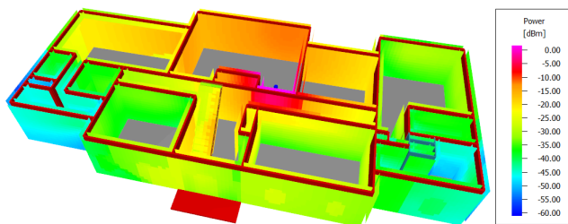
Figure 50: An example of a building with predictions along surfaces.
