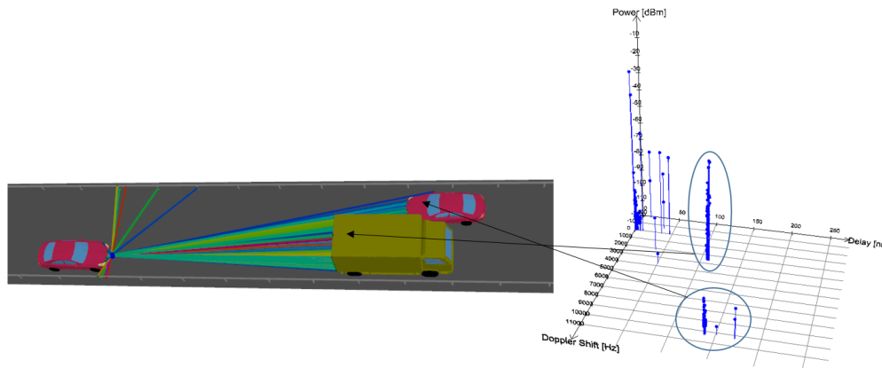
Figure 78: An automotive radar simulation in Altair WinProp.
