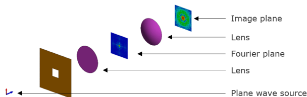
Figure 70: The optical 4F correlator (dielectric lenses) in the image simulates 16 times faster in Feko 2019 than in Feko 2018.2.1 on a laptop with Nvidia Quadro M1000M GPU.
