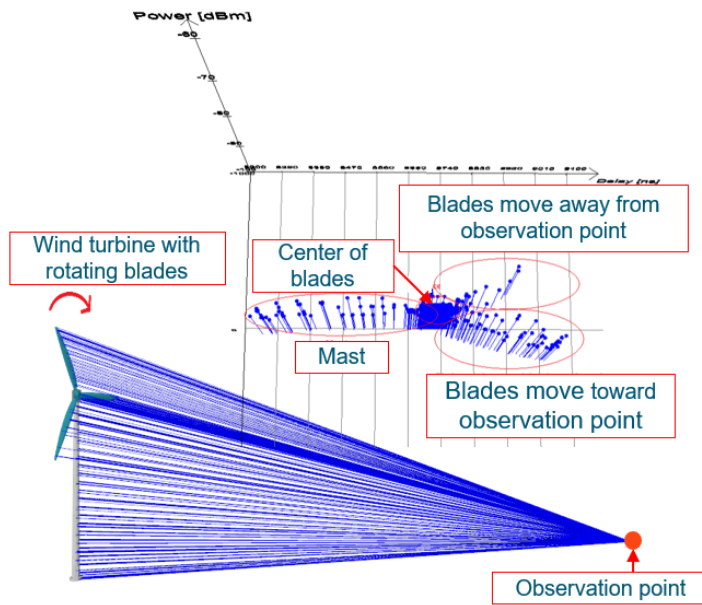
Figure 38: Calculation of Doppler shift due to the rotation of the blades of a wind turbine.
