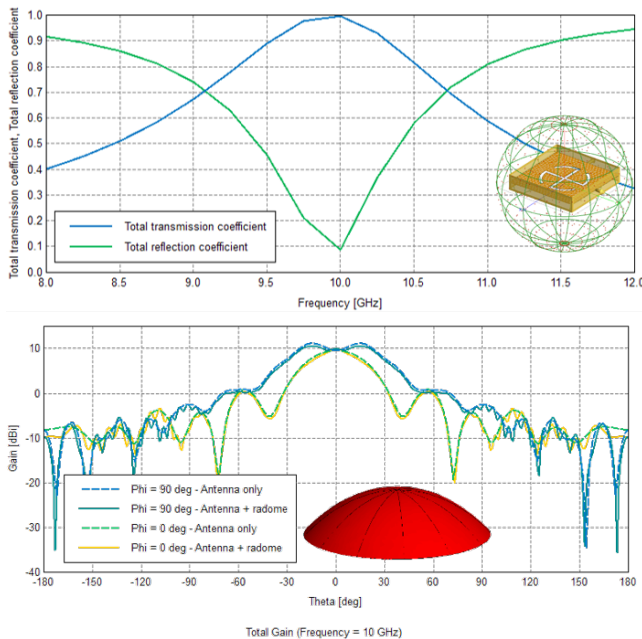
Figure 83: Antenna operating at 10 GHz with FSS radome modelled with a characterised surface. The radome simulation completes within a few minutes.
