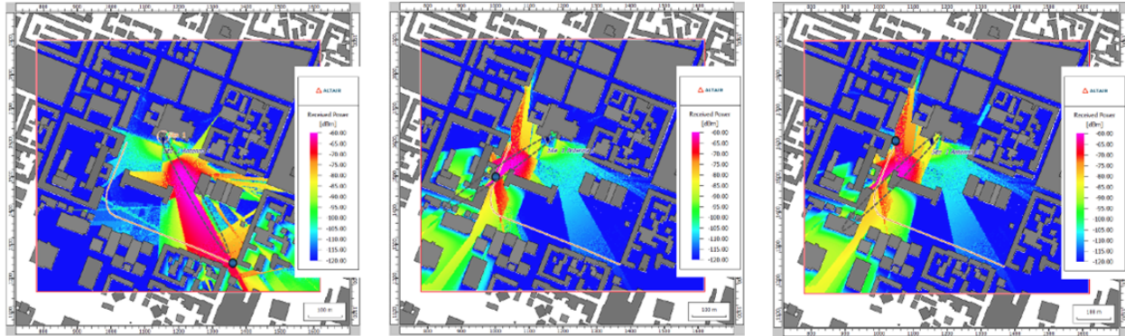
Figure 3: Left: Only the data beams that are serving a user are active (the best serving beam is selected). Centre: If the user moves, it switches to another predefined beam. Right: The serving beam is not necessarily oriented in the direct direction, it can for example, come from a reflection at the building.
