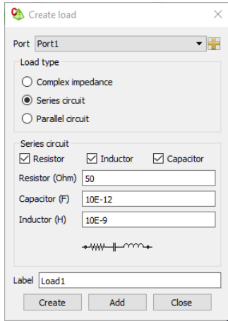
Figure 76: The Create load dialog now shows an image of the resulting circuit.
