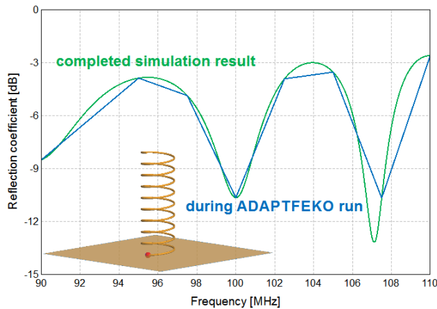
Figure 87: A Cartesian graph with the reflection coefficient of a helix antenna shows the completed continuous frequency result and the discrete result as it gets displayed during simulation.
