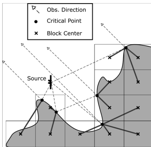
Figure 46: Using ray-tracing to determine critical points and optimize the number of macro-basis functions needed per block for a specific source point and observation direction in a solution using the CBFM.
