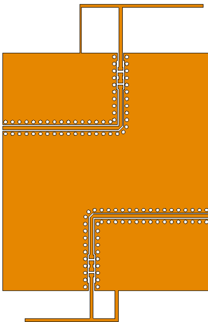
Figure 81: View of an exported Gerber file of a planar antenna with via holes.
