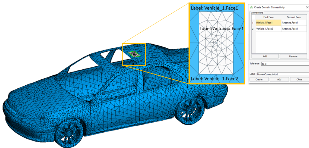
Figure 8: A static imported car mesh and a parameterised antenna geometry viewed in POSTFEKO where the Domain Connectivity display tool highlights edges in green that are connected using domain connectivity.
