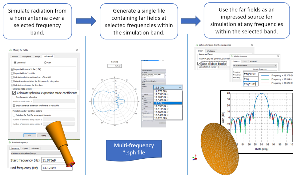
Figure 47: Using a spherical mode representation of a horn antenna pattern as an impressed source for a parabolic reflector to calculate radiation patterns at flexible frequencies.
