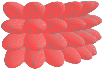
Figure 58: Envelope pattern generated in AMan.
