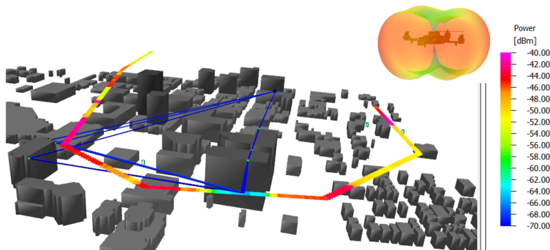
Figure 64: An illustration of a virtual flight test as an example of a 3D trajectory in an urban scenario.
