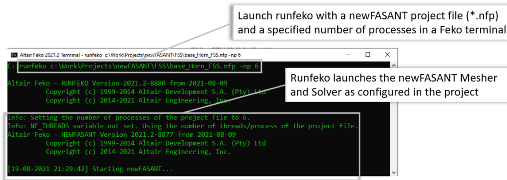
Figure 45: Meshing and solving a newFASANT project from the Feko terminal using a standard runfeko command.
