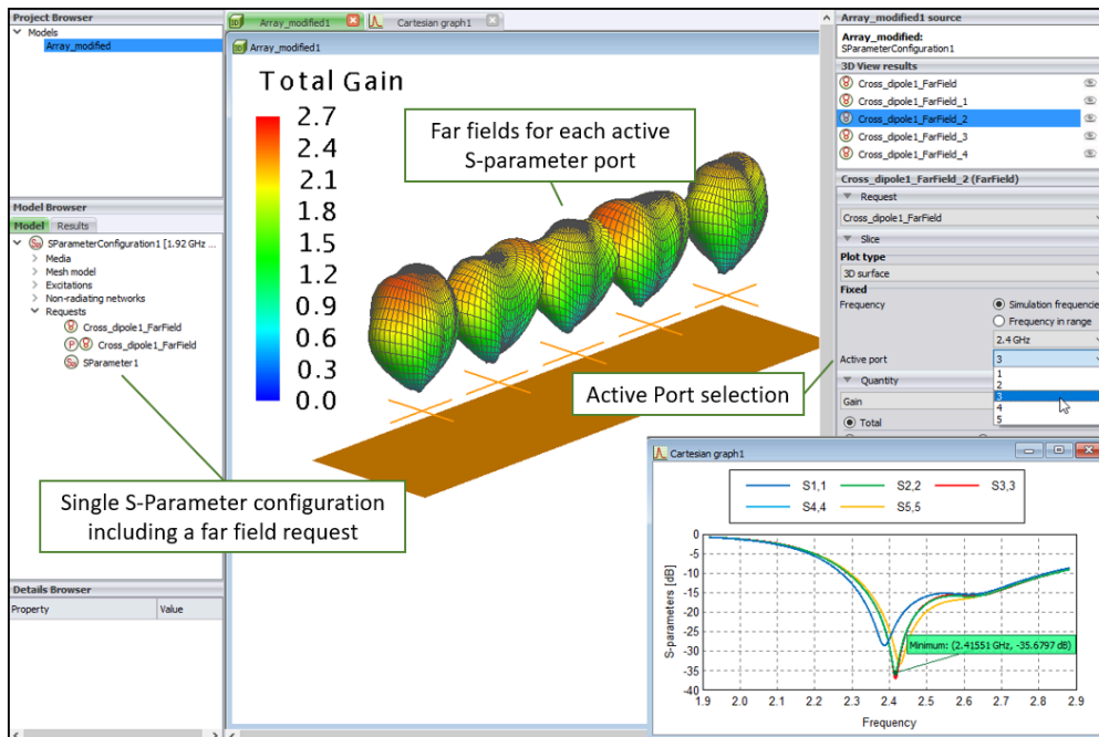
Figure 41: A cross dipole array illustrating the visualisation of the embedded element radiation patterns calculated as part of a single S-parameter configuration.
