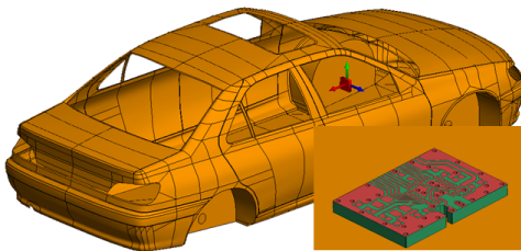
Figure 61: A PCB simulated in PolEx can be included as a source in a Feko simulation.
