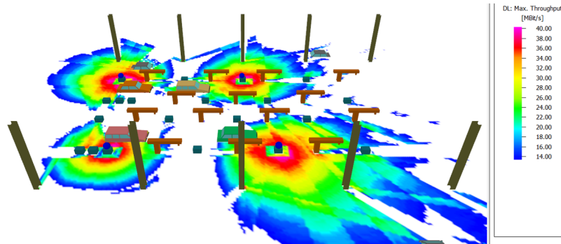
Figure 62: Co-existence between Bluetooth and Wi-Fi in a factory hall.
