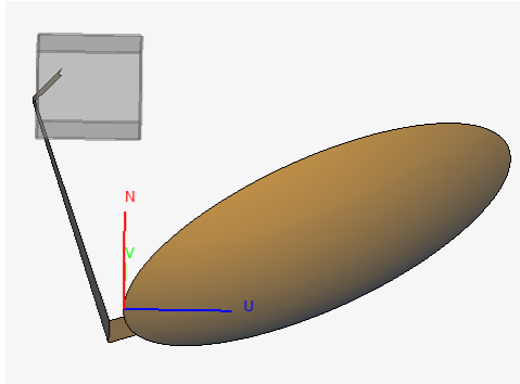
Figure 29: An offset reflector with an imported protected model of a horn (feed) showed in grey in CADFEKO.
