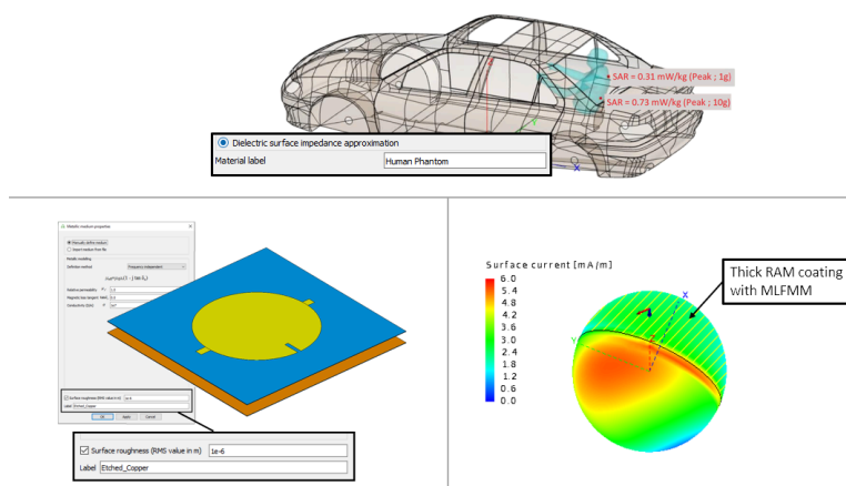
Figure 53: New surface modelling options enabling fast SAR calculation, consideration of metal surface roughness effects and simulation of thick, high-loss dielectric coatings for RAM applications.
