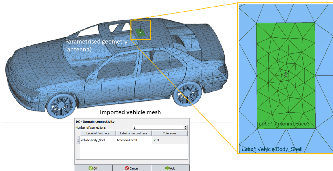
Figure 15: An installed performance study using a static imported car mesh and a parameterised antenna geometry. Though there are no shared mesh vertices between the car roof and the antenna ground plane, the roof and antenna ground plane will be treated by the MoM/MLFMM Solver as if “connected” based on the Domain Connectivity specified in a DC card.
