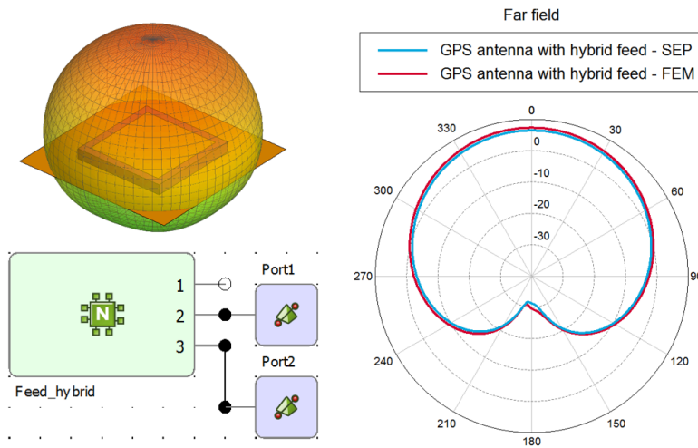
Figure 66: A GPS antenna with feed network solved with the MoM (SEP) and the FEM.
