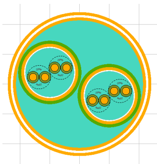
Figure 75: CADFEKO cross-sectional view of a cable bundle with double shields.
