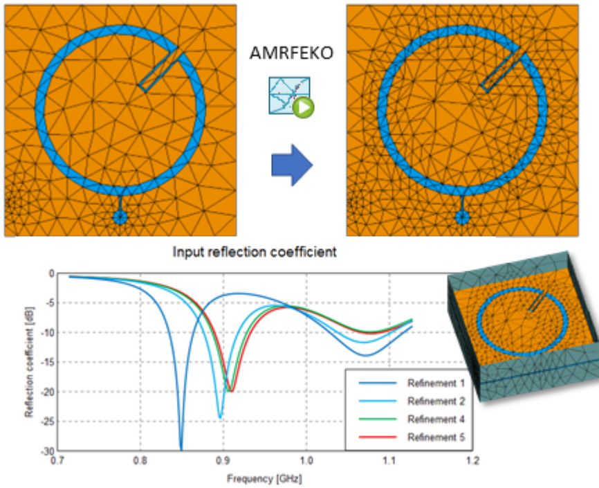
Figure 7: An example of a model refined using AMRFEKO; Left: unrefined, Right: final refinement.
