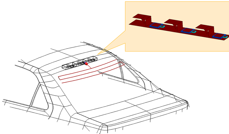
Figure 80: Partial view of a car with a windscreen antenna solved with the MoM/MLFMM and an antenna module mounted in the car's roof (shown enlarged in the insert) solved with the FEM.
