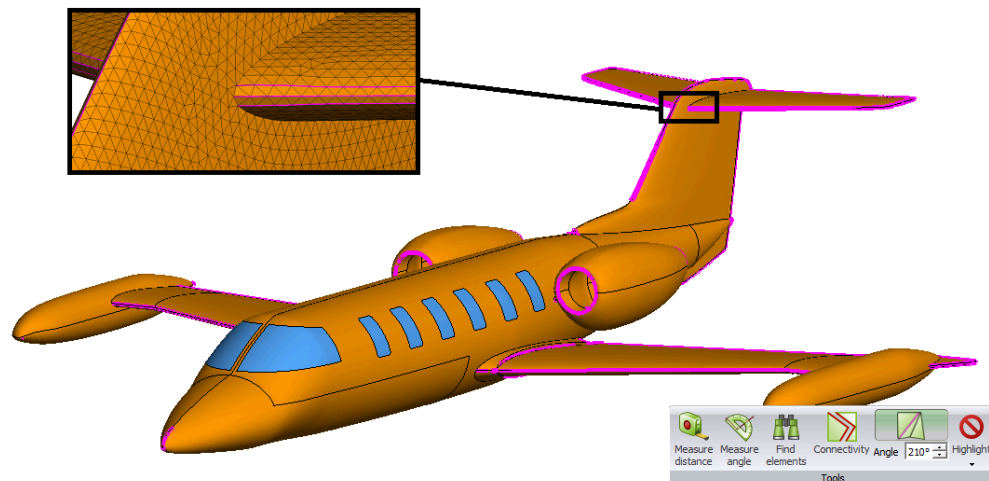
Figure 40: Highlighting mesh elements in POSTFEKO where the angle between the elements exceeds a threshold.
