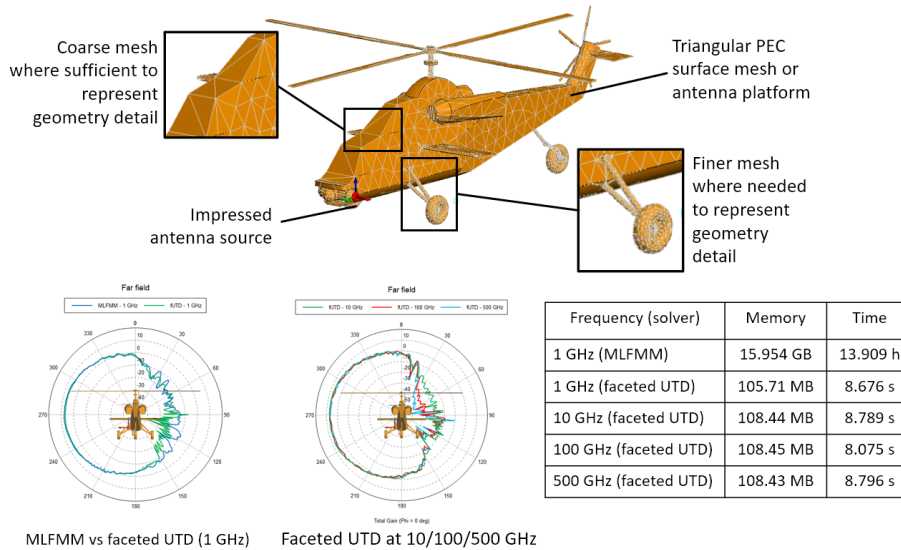
Figure 49: New faceted UTD solver added to Feko for frequency-independent antenna placement analysis.
