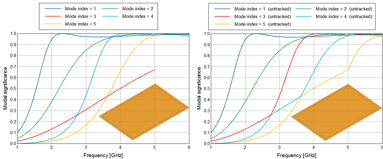
Figure 88: Modal significance plots from a characteristic mode analysis performed on a PEC plate showing tracked modes on the left and untracked results on the right.
