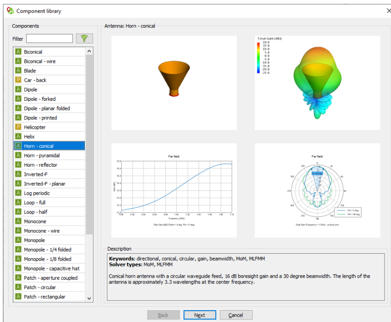
Figure 63: The new component library.
