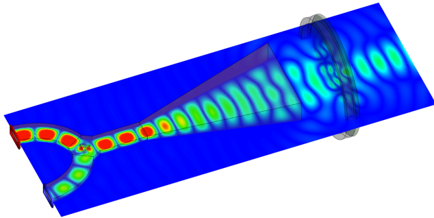
Figure 84: Ferrite circulator (FEM) with horn antenna and dielectric lens (SEP).
