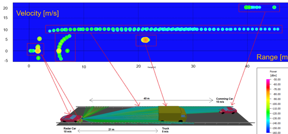
Figure 55: An example of a heat map for automotive radar.
