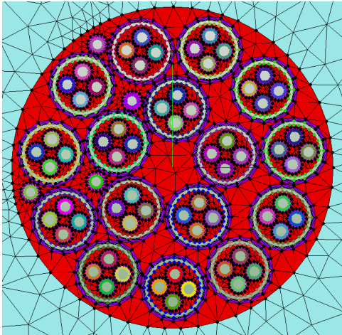
Figure 86: An example of a cable cross section mesh used by the solver.
