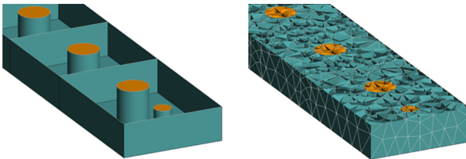
Figure 89: Partial view of a coaxial diplexer model (left) and mesh (right) with the perfect electric conductor pins meshed into tetrahedra with the dielectrics and solved as part of the FEM solution.
