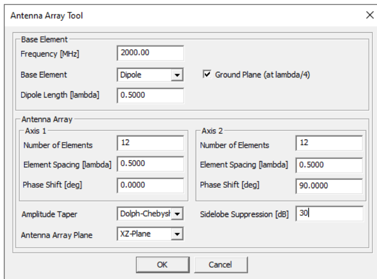
Figure 30: The Antenna Array Tool dialog where you can define rectangular array elements.
