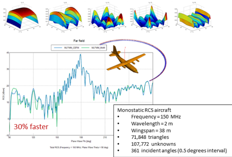
Figure 9: An example of a monostatic RCS calculation of an aircraft solved with MLFMM and MoM/MLFMM.
