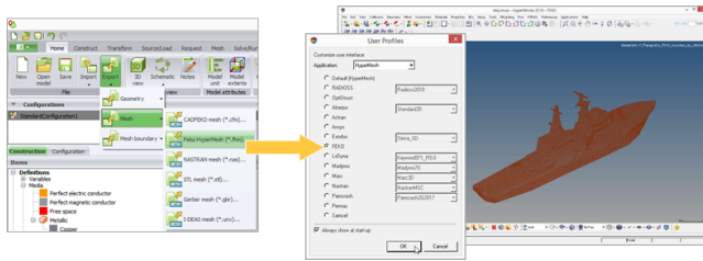
Figure 72: The Feko User Profile in HyperMesh ensures the generation of a valid mesh for Feko.
