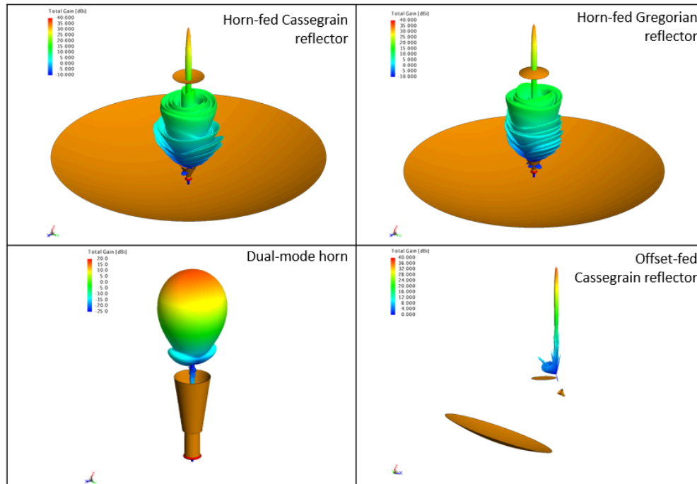
Figure 22: The four new components added to the Component Library.
