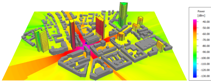
Figure 51: An example of an urban scenario with predictions along building surfaces.
