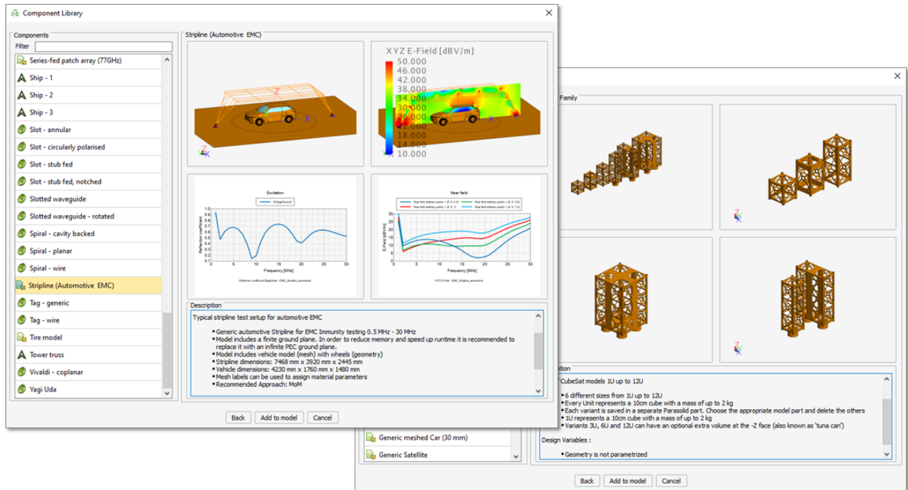
Figure 6: A selection of the new components available in the component library.
