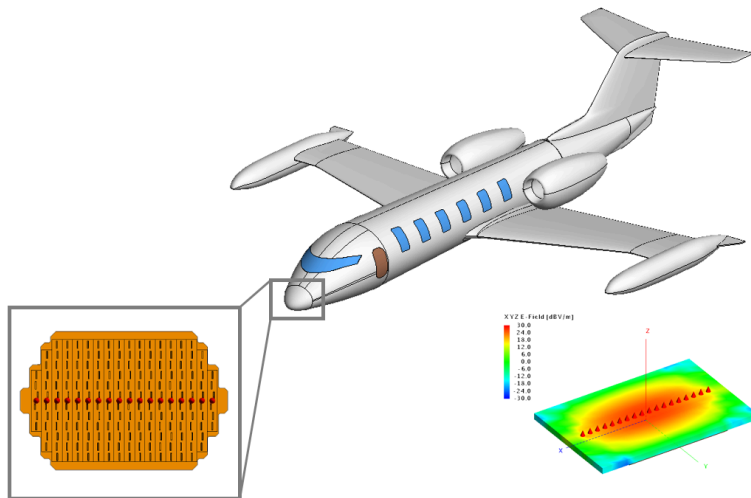
Figure 65: An example of a weather radar in an aircraft radome where the Cartesian boundary near field request can be used to simplify model decomposition.
