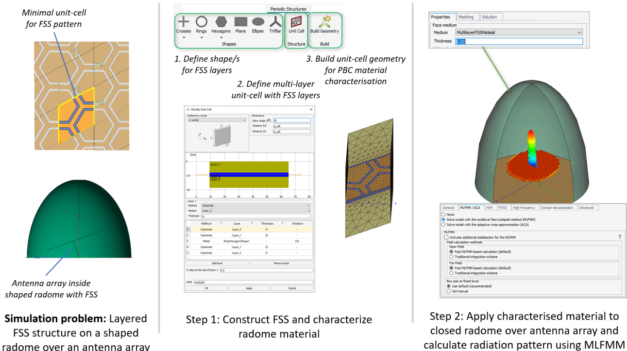
Figure 21: A streamlined and flexible workflow for simulation of multi-layer FSS radome structures using material characterisation with PBC and MoM/MLFMM.
