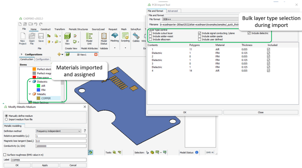
Figure 23: During import of PCB formats materials are included and assigned. In addition bulk include/exclude of layer types is supported.
