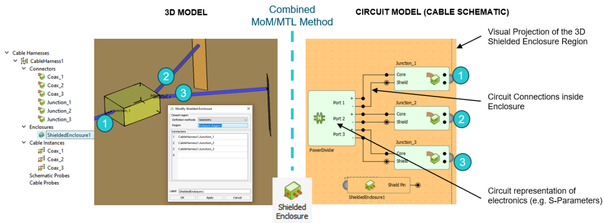
Figure 1: Illustration of the new shielded enclosure functionality in Feko.
