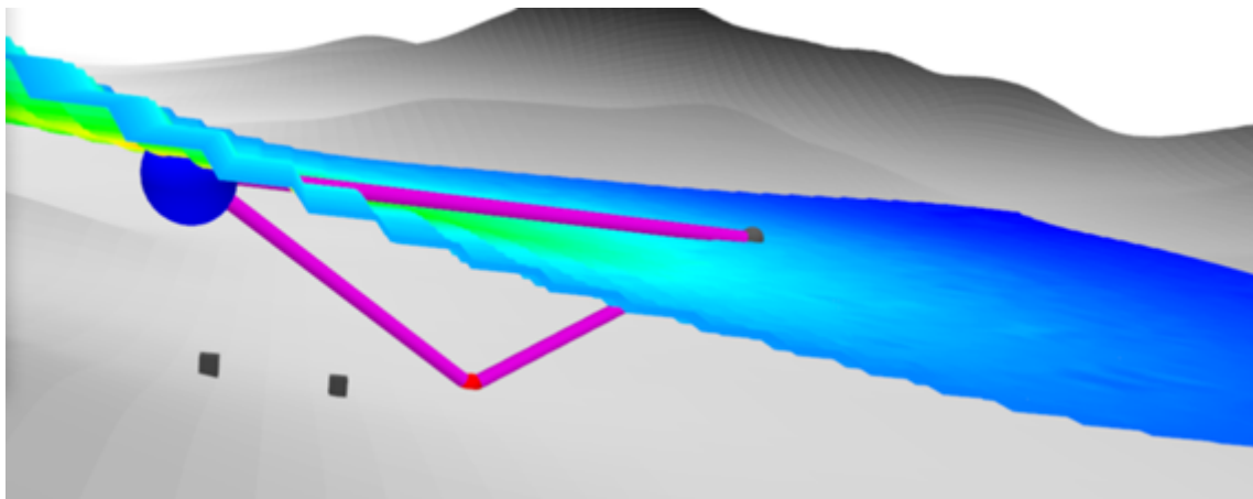
Figure 26: An example of a ground-reflected ray using Urban Intelligent Ray Tracing.
