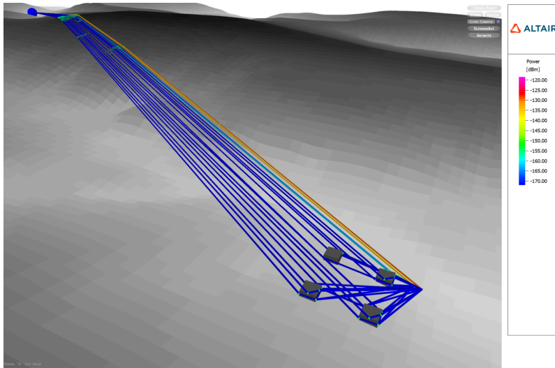
Figure 31: 3D multipath in an urban scenario where the transmitter is shadowed from the buildings due to hilly terrain.
