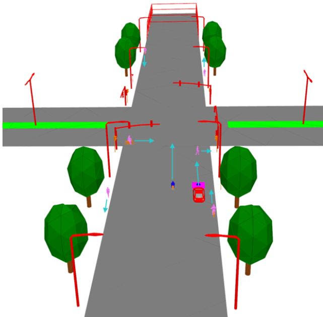
Figure 32: The library contains useful traffic objects that can be used to simulate the performance of automotive radar in traffic.
