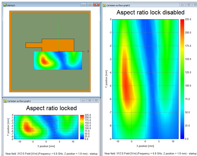
Figure 67: The aspect ratio of a surface graph can be locked.
