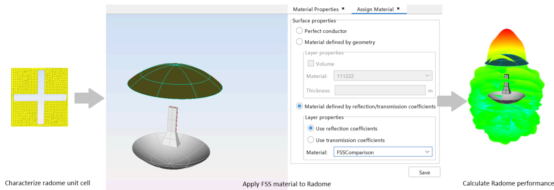
Figure 39: The new workflow for accurate and fast characterisation of multi layer radomes with FSS performance based on pre-characterisation of the radome and FSS as a material.
