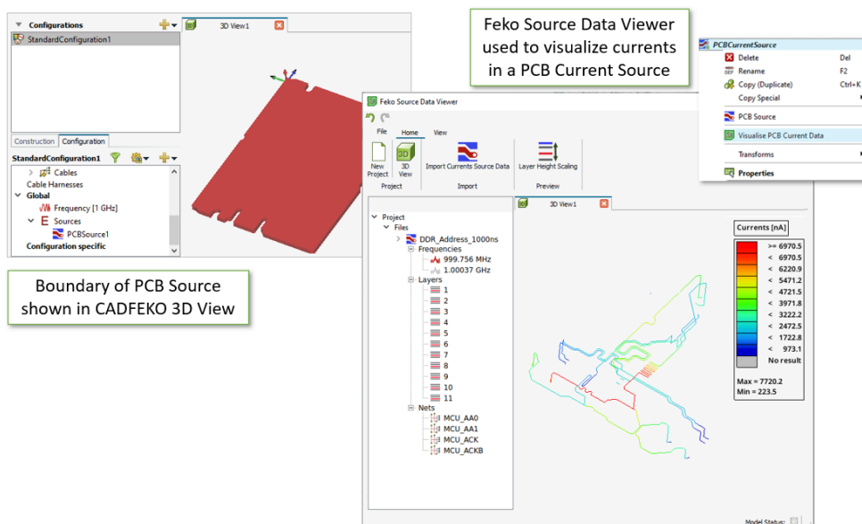
Figure 24: Viewing the boundary of a PCB Source and using the Feko Source Data Viewer to view the currents included in a PCB source at a chosen frequency.
