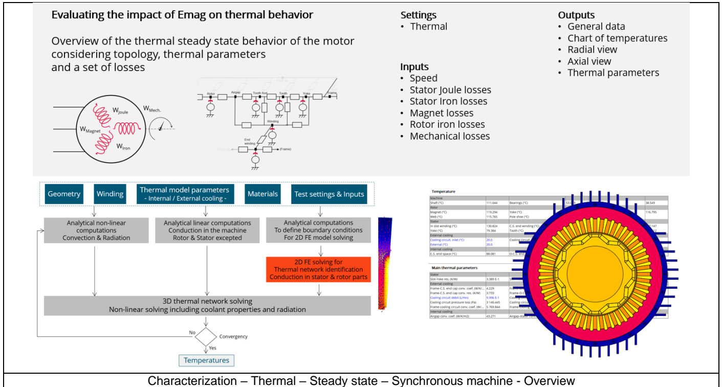
Characterization – Thermal – Steady state – Synchronous machine - Overview
